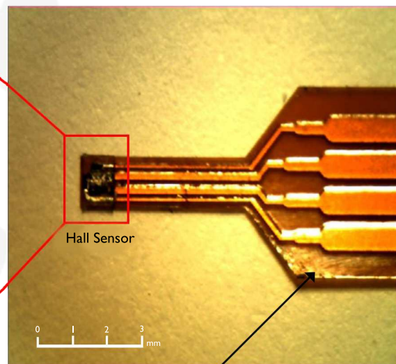
Flex PCB
